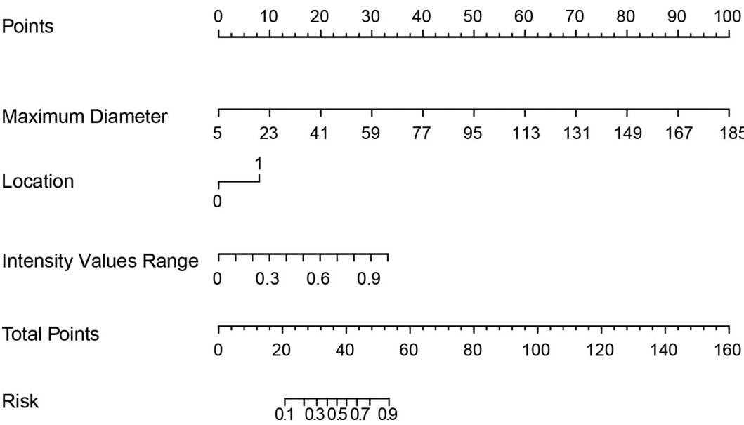
Figure 4. Developed radiomic nomogram. The radiomic model, maximum diameter, range, and tumor location were used for building the radiomic nomogram. The probability of each predictor can be converted into scores according to the first scale “Points” at the top of the nomogram. After adding up the corresponding prediction probability at the bottom of the nomogram is the malignancy of the tumor. The cutoff point of our nomogram is 0.5. The case would be diagnosed as high malignant potential when the total prediction probability is beyond the cutoff point.
